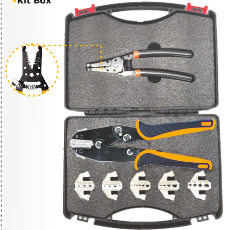
COAXIAL CRIMPING TOOL-RG58,59,62,8X,140,142,174,210,223,303,400, FIBER OPTIC, BELDEN 8279 CX-02
