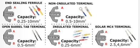
OPEN BARREL TAB TERMINAL (TAB 2.8,4.8,6.3) CRIMPING TOOL JN 48B
